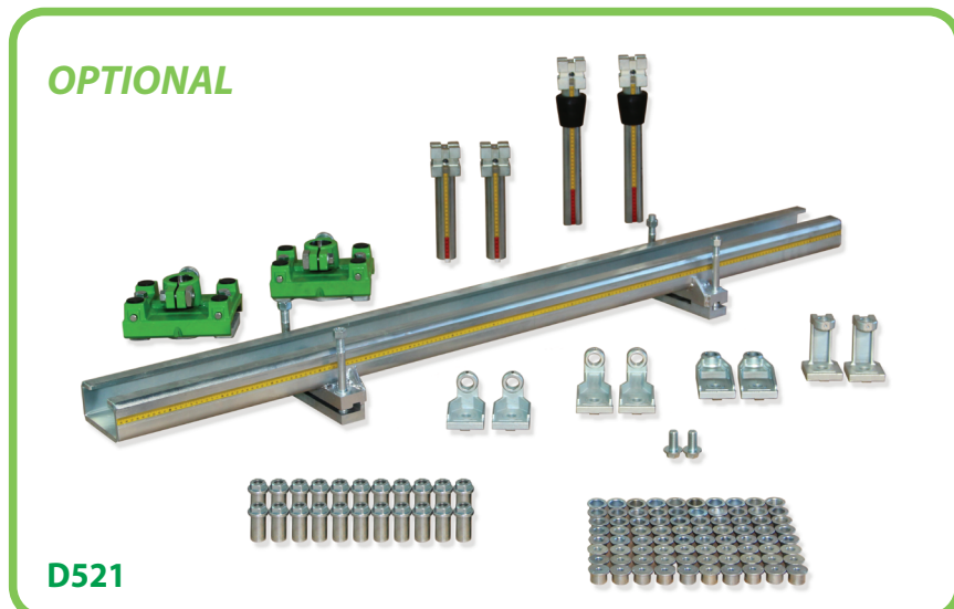
New GLOBALJIG accessory kit, very useful for fixing and sealing the parts of the vehicle to be welded or replaced, or to make comparison measurements with the non-affected part of the vehicle.
